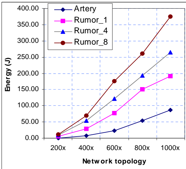
Figure 5. Energy Consumption. For clarity, we only show Rumor routing with three variants of number of agents per event.
