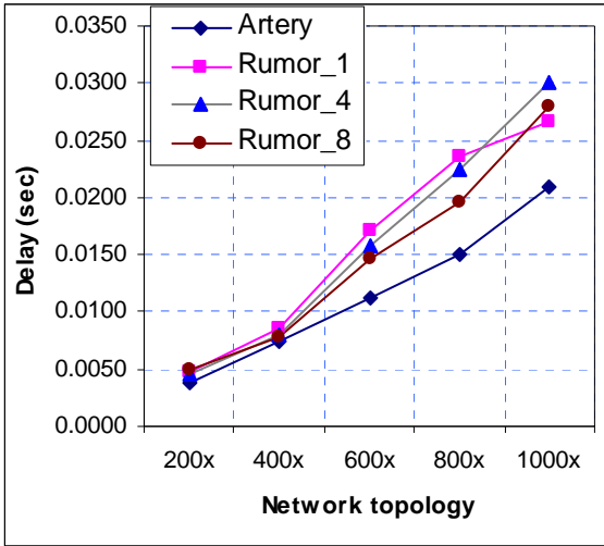
Figure 4. Delay comparison.
